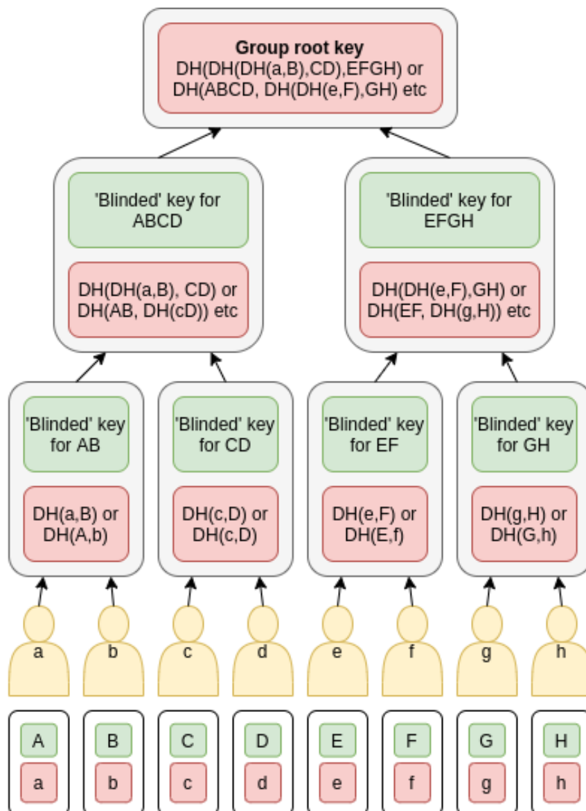
Figure 16: A key tree. Secrets are shown in red boxes, and only obtainable by members below them in the tree. The associated 'blinded' keys (green) are distributed to other group members such that all members can compute the root key
