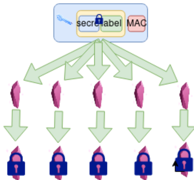
Figure 1: Diagram from the protocol specification showing the backup process. The encrypted secret together with its key is distributed into shards. The shards are encrypted for each custodian.
