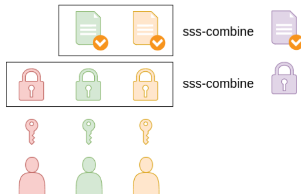
Figure 15: BLS Threshold signature - Here, 2 of 3 members' signatures are combined to give a group signature. The group public key is the same regardless of which members signed
