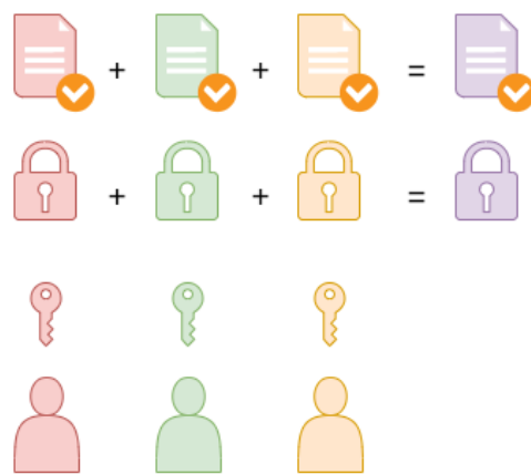
Figure 14: BLS Signature aggregation - if public keys and signatures are added together we get an aggregate signature with can be validated with the corresponding aggregate public key
